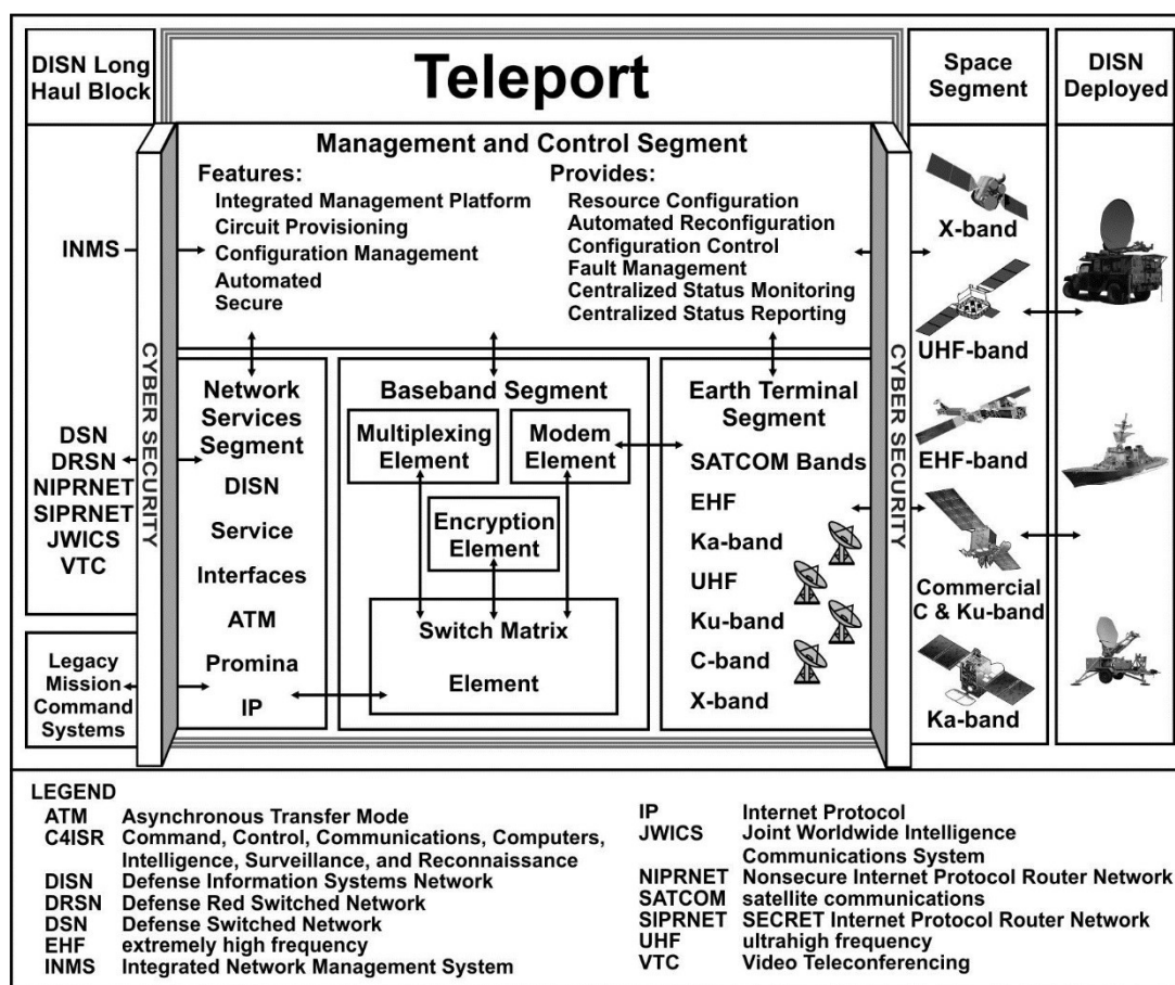
Figure A-2. Teleport program
