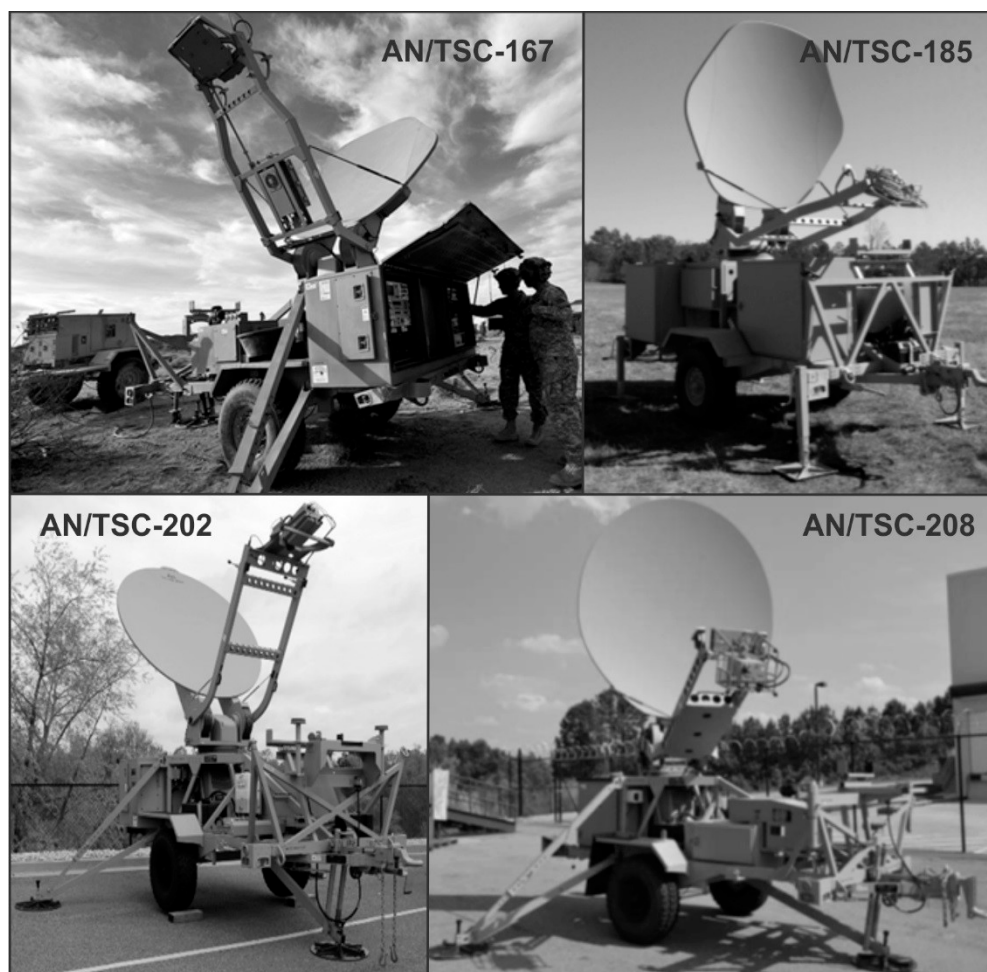
Figure A-16. Satellite portable terminal
