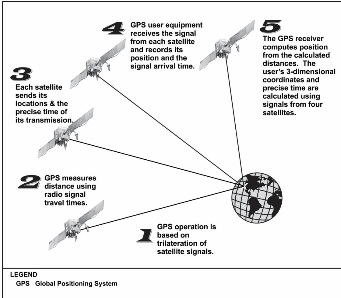
Figure B-1. How the global positioning system works
