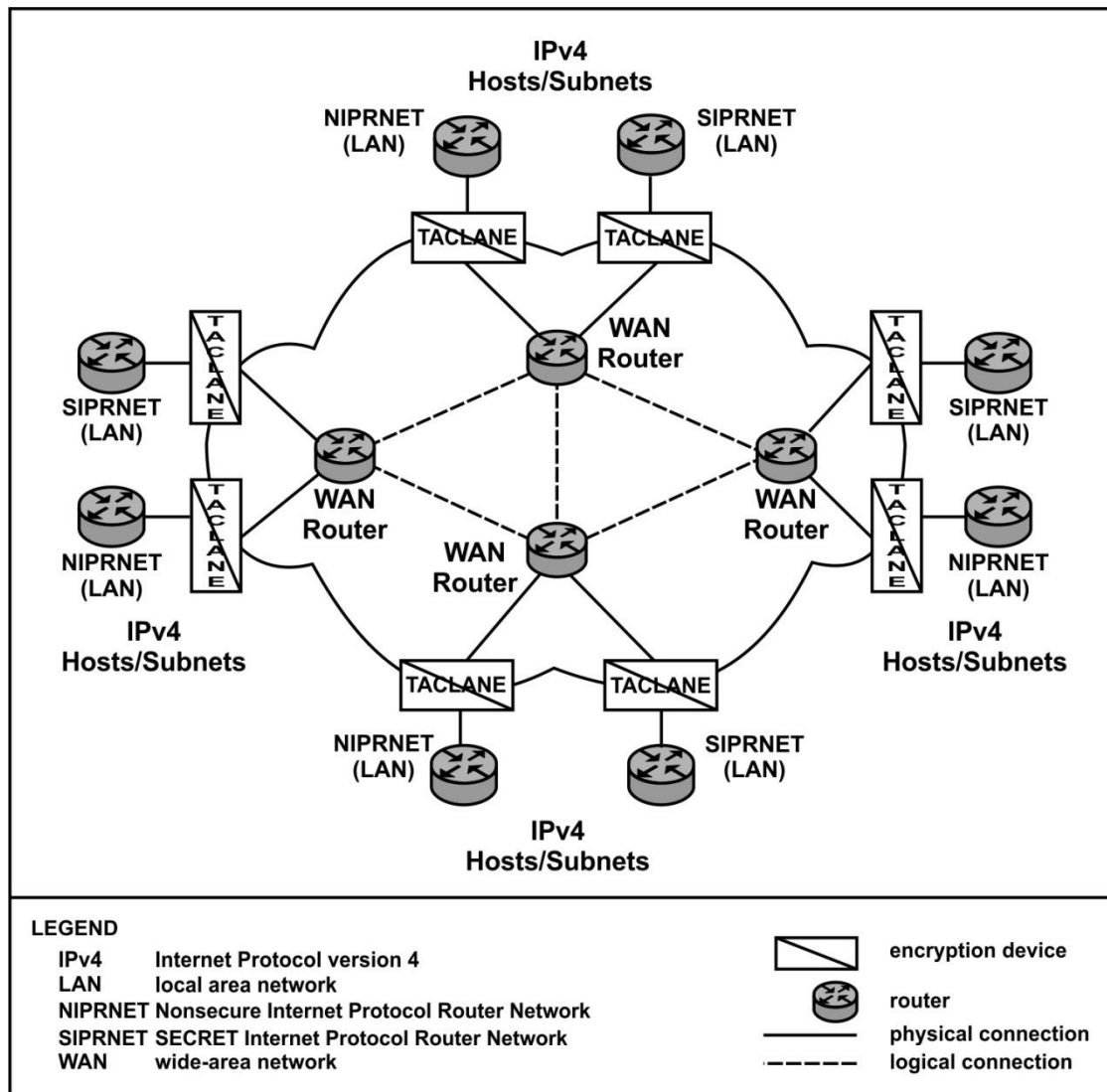
Figure 3-5. Colorless core routing
