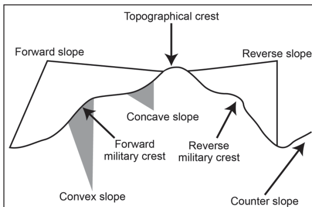
Figure 6-6. Slope terminology
